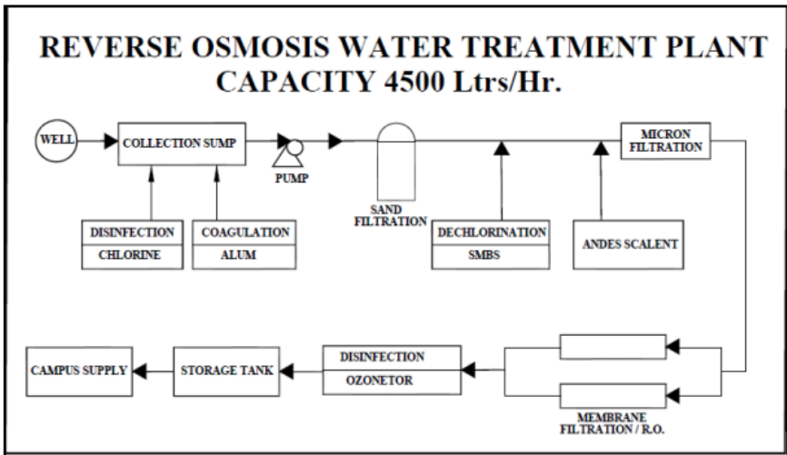
FLOW CHART FOR THE RO PROCESS
